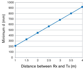
Mounting position (20 elements)
