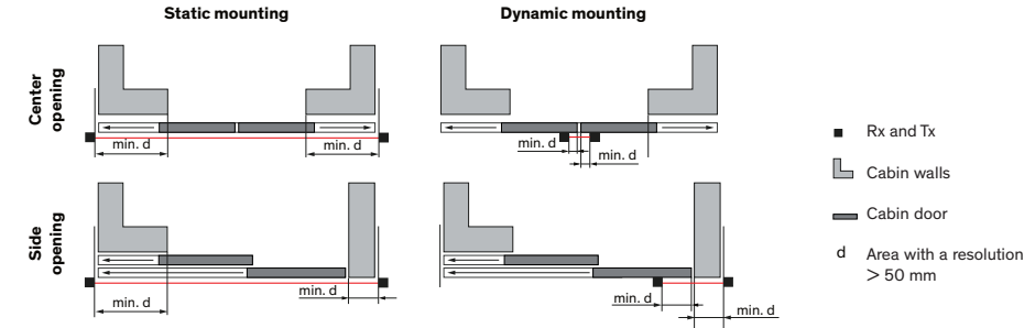
Mounting position (20 elements)
