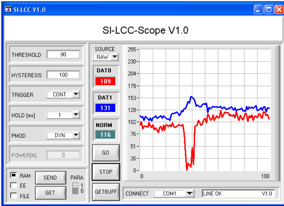
Windows® user interface
