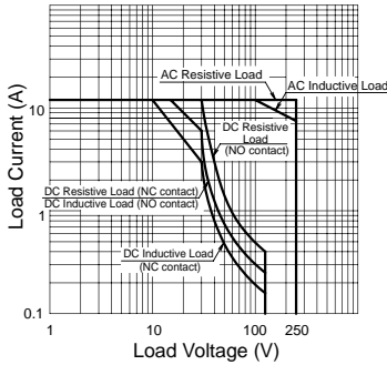
RJ1V Plain
