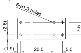
RJ22V-A-*
