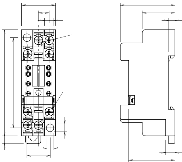
Terminal Arrangement
