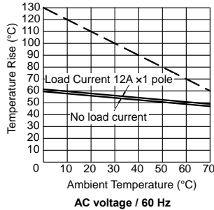
RJ2V Plain
