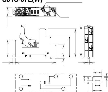
SJ1S-07L(W)
