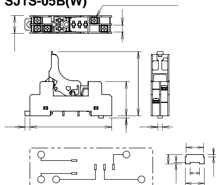
SJ1S-05B(W)
