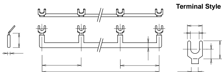
Terminal Style
