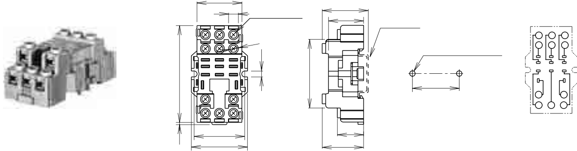
SH4B-05A
