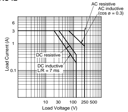
RU42
