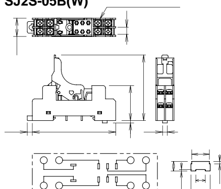
SJ2S-05B(W)
