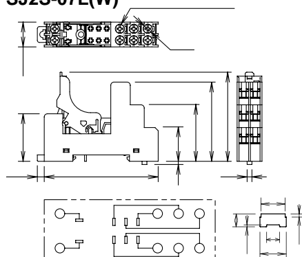
SJ2S-07L(W)
