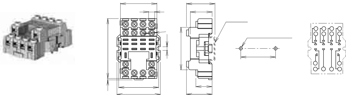
SH4B-05C
