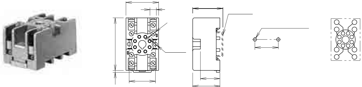
SR2P-05C
