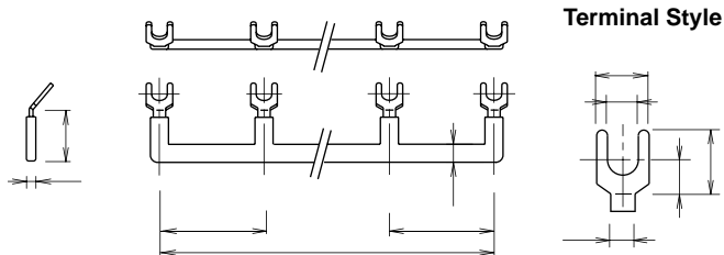
Terminal Style
