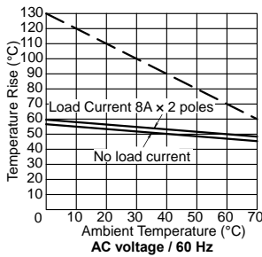
RJ2V Plain
