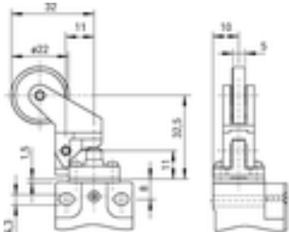
Plastic roller lever with collar 4K
