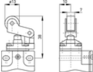
Metal roller lever with collar WHM
