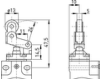
Offset metal roller lever with collar WHKM
