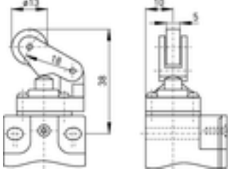
Roller lever with collar WH
