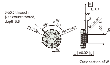
Load cell tip mounting jig reference size
