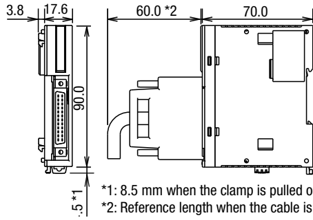
FC5A-EXM1M
