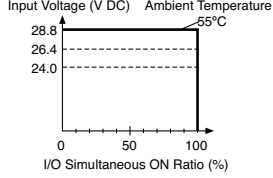
FC4A-N08B1
