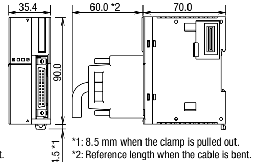
FC5A-EXM1S
