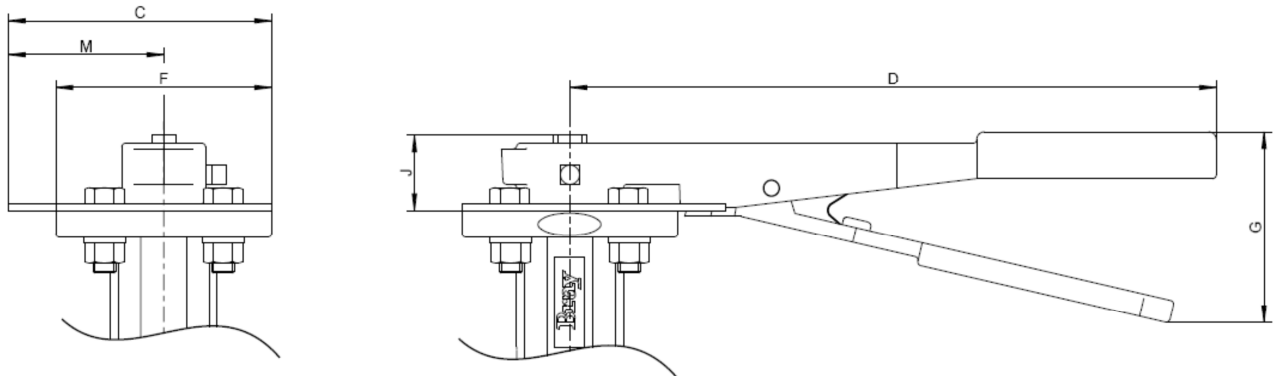
Fig. 4 Operating lever DN 50 to DN 300 with lockable notch plate
