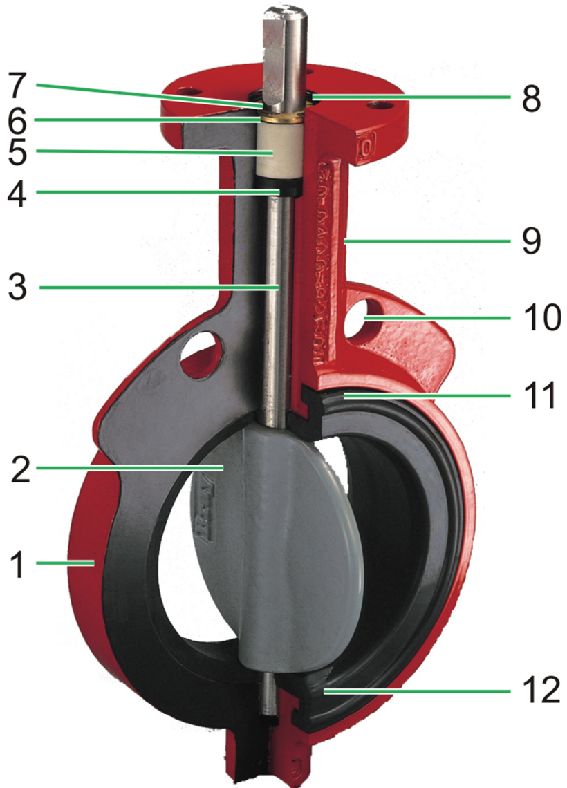
Fig. 1 Example Butterfly Valve Sectioned
