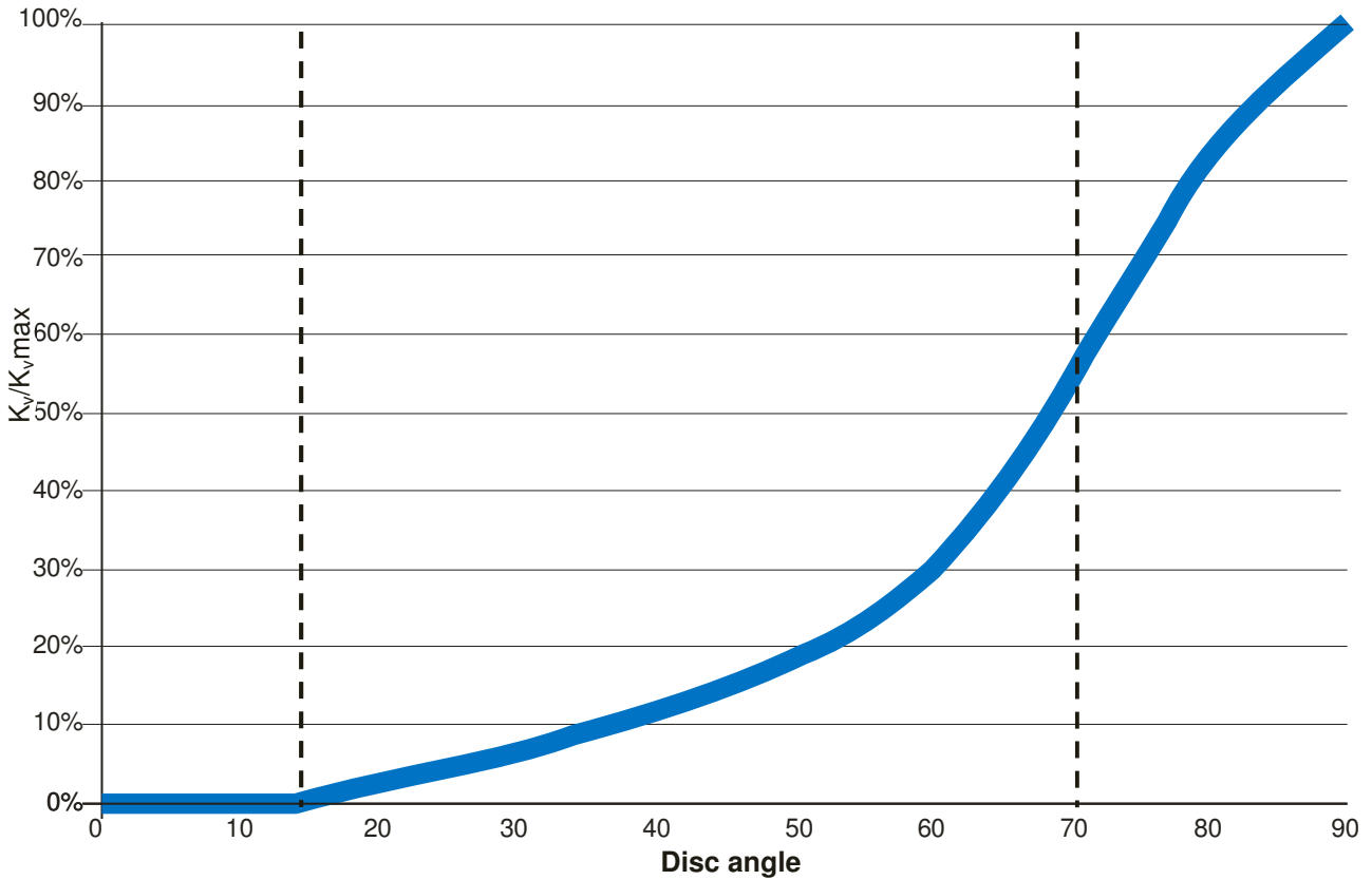
Fig. 3 BV 10000, flow curve, schematic diagram, DN50 up to DN 500
