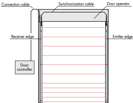
Figure 6: GridScan/Mini-SB2/-ST2 application (overview)
