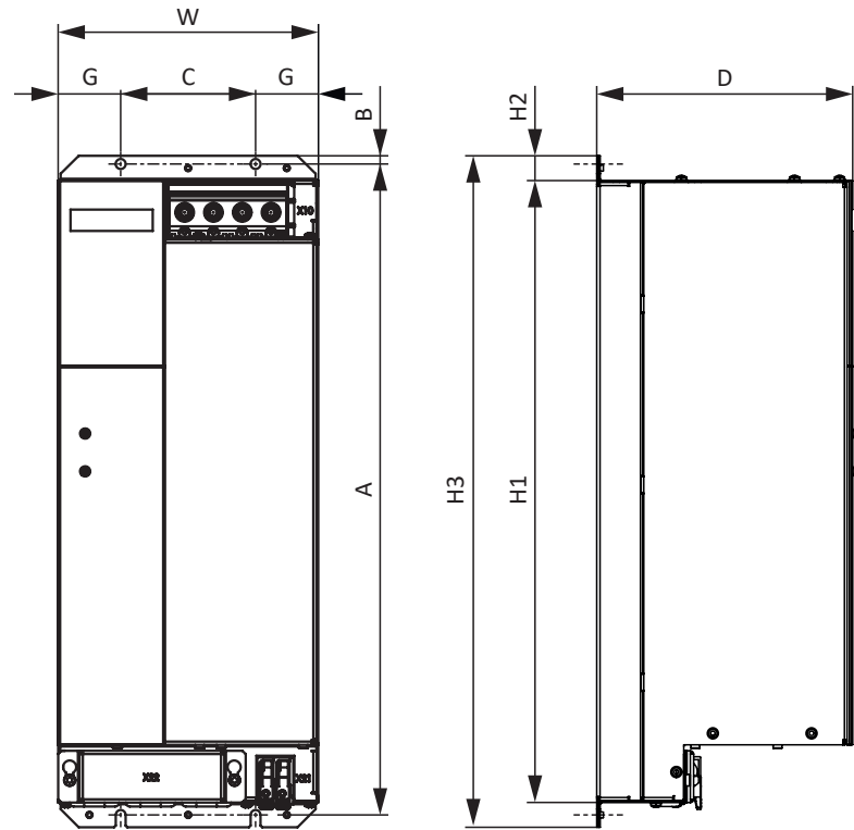
Fig. 4: PS6A44 dimensional drawing
