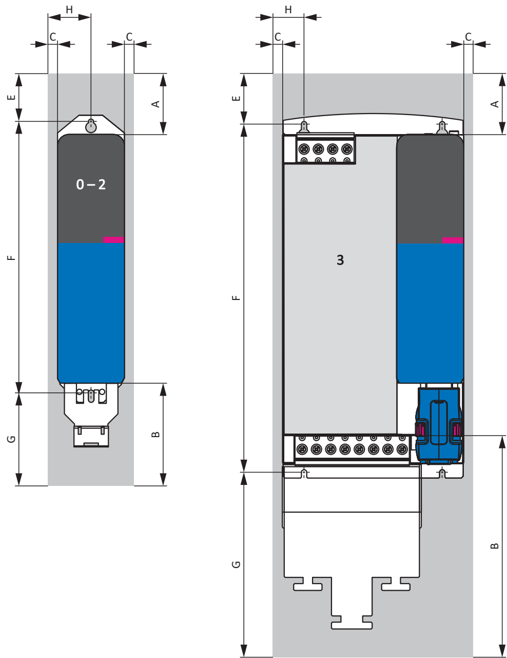
Fig. 3: Minimum clearances
