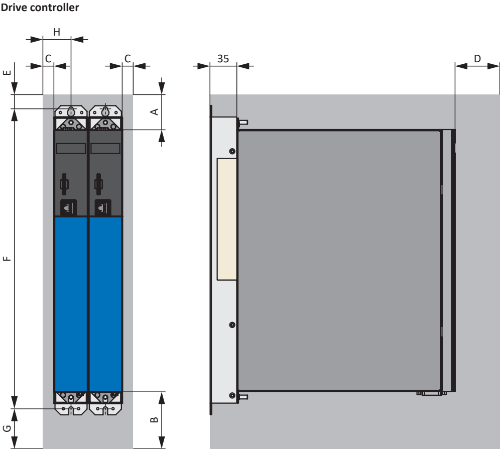
Fig. 3: Minimum clearances
